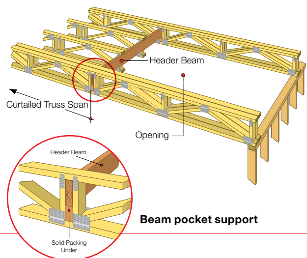
Fig 31 - Floor openings.
