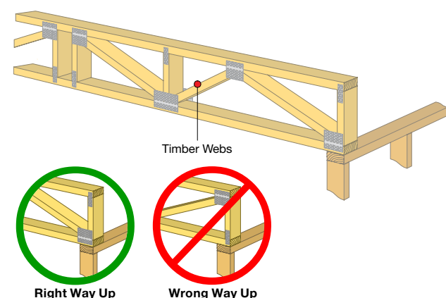
Fig 1 - Longreach truss.
