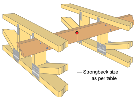
Fig 40 - Longreach Strongback.
