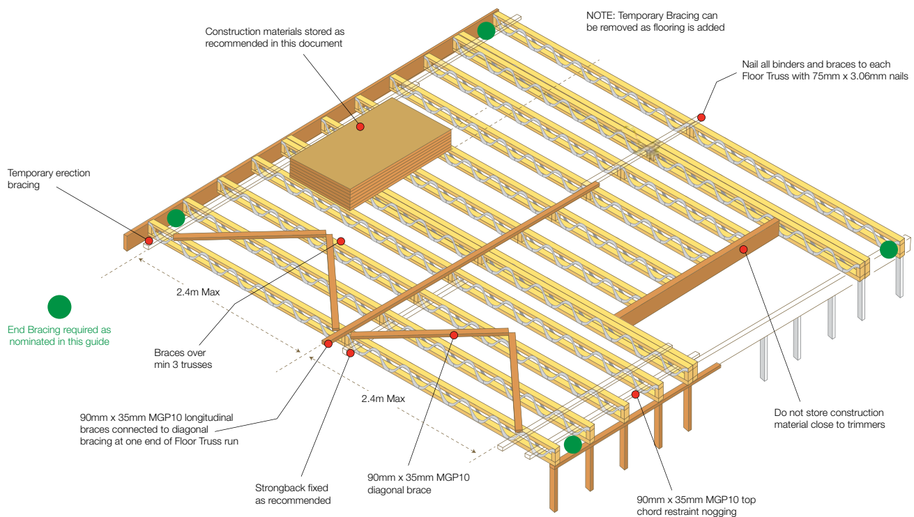
Fig 6 - Bracing.
