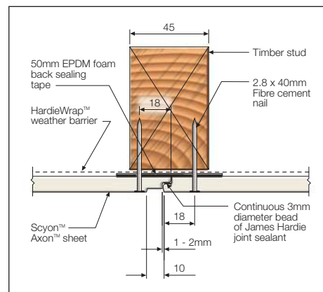
FIGURE 11 FIBRE CEMENT NAIL FIXING
