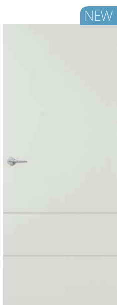
MOTP 2 Prime
